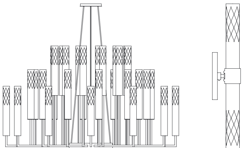
CHANDELIER Dia 1060 mm × H 880 mm
